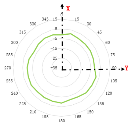
Azimuth plane (top view) - 5GHz
