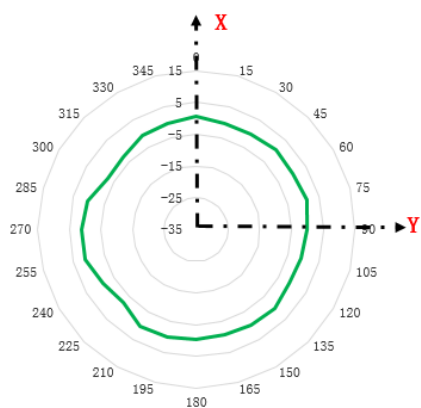
Figure 1. AP361 antenna pattern plots Azimuth plane (top view) - 2.4GHz
