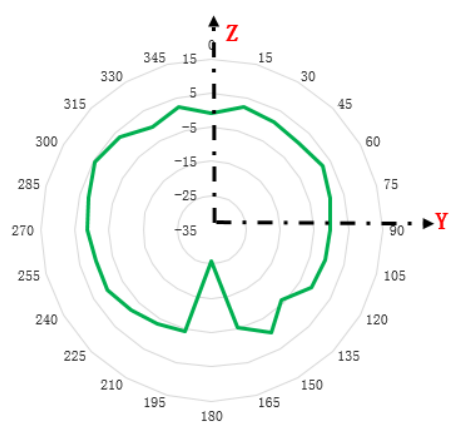
Elevation plane (side view,90 degrees)-2.4GHz
