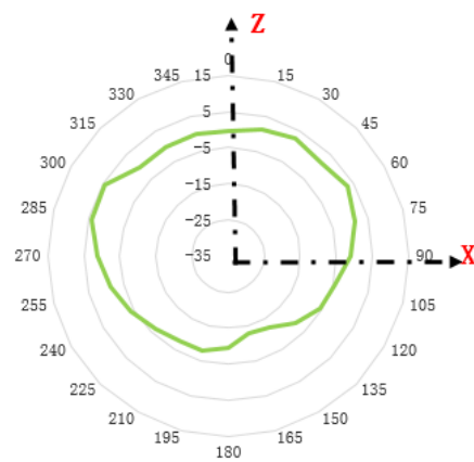
Elevation plane (side view,90 degrees)-5GHz
