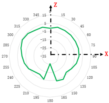
Elevation plane (side view,90 degrees)-2.4GHz
